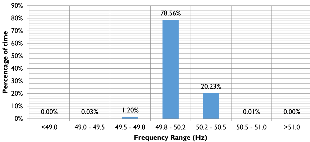
Figure 2.9: System Frequency for 1 st half of 2020
