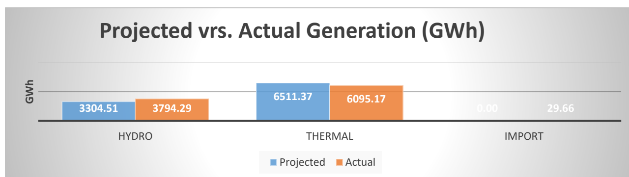
Figure 2.5: Projected versus Actual Energy Generation for 1 st half of 2020
