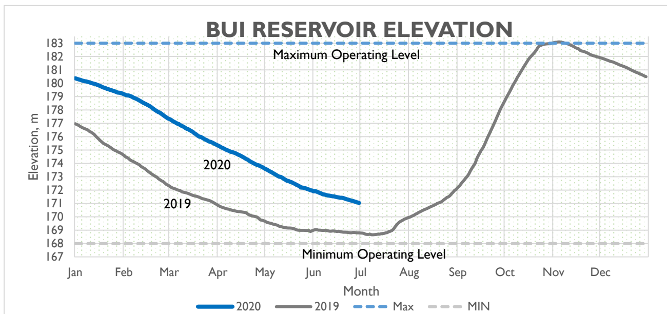
Figure 2.8: Bui Reservoir Trajectory
