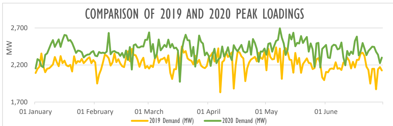
Figure 2.3 2020 vs 2019 monthly peak loadings
