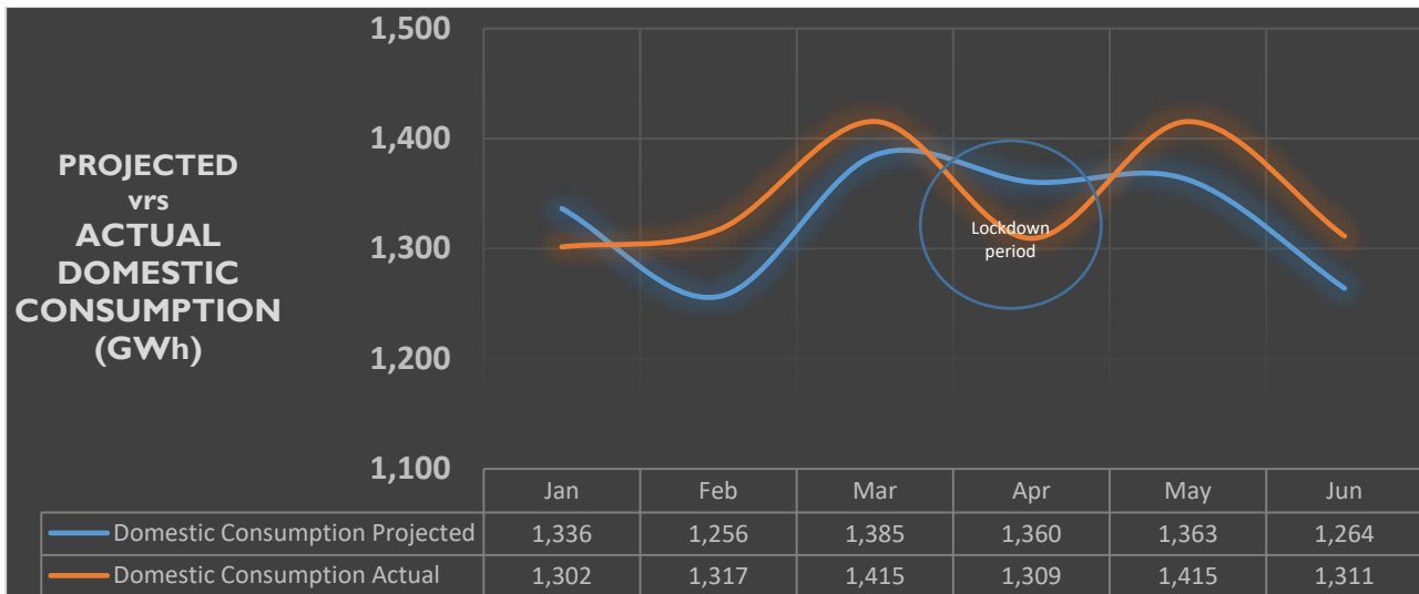
Figure 2.2 Projected vs. Actual Domestic Energy Consumption in 1st half of 2020
