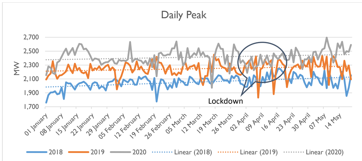
Figure 2.1 Daily domestic peak demand January 1 – May 19 for 2018, 2019 and 2020
