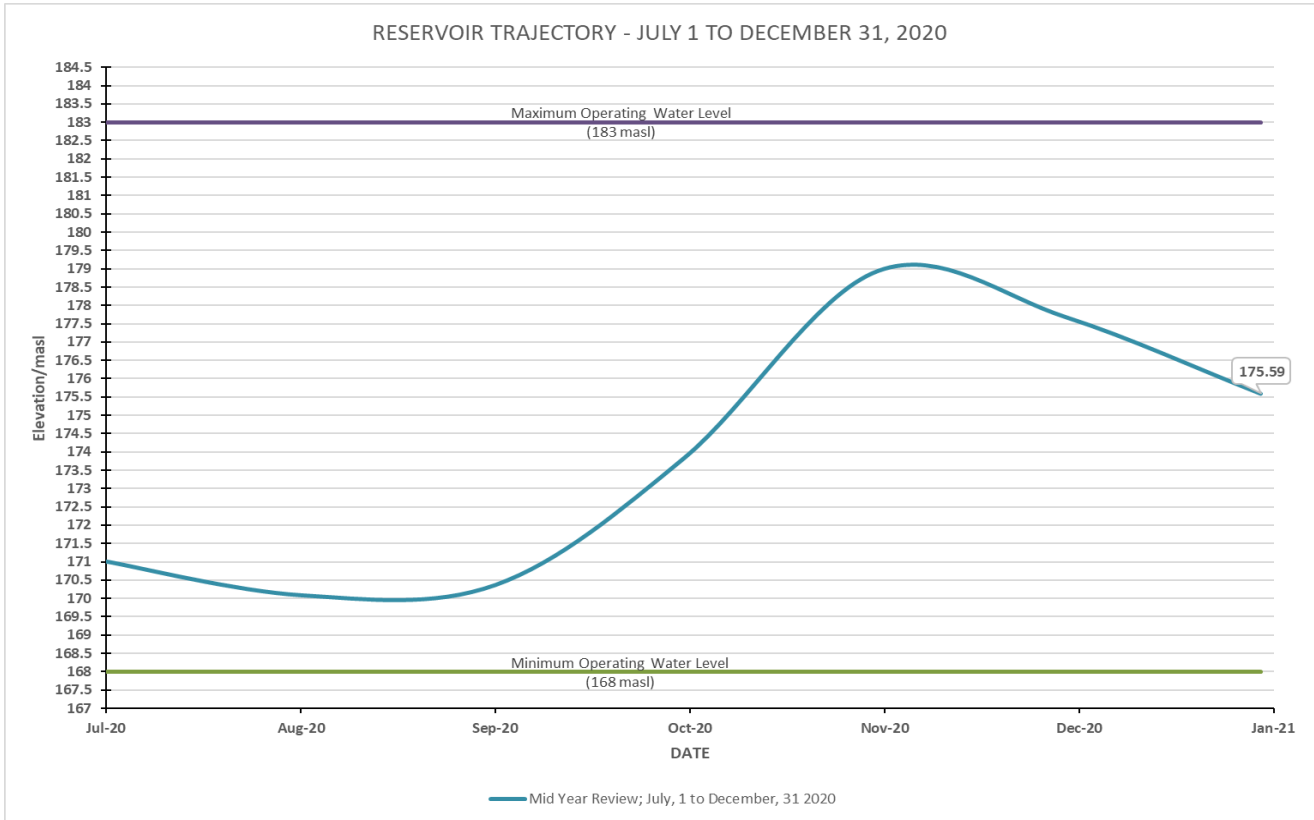
Figure 4.2: 2020 Projected Bui Reservoir Trajectory
