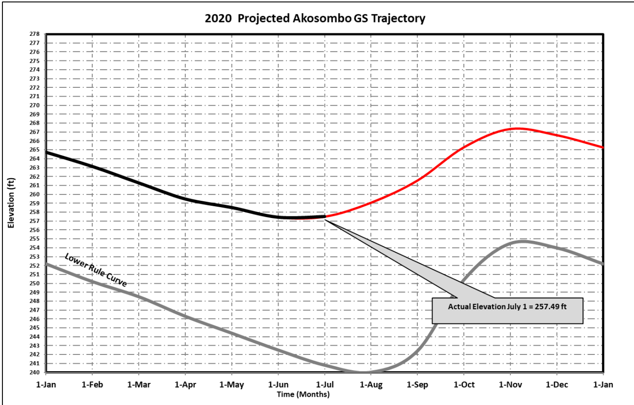
Figure 4.1: 2020 Projected Akosombo Reservoir Trajectory
